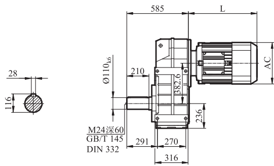
GFA/GFH127
