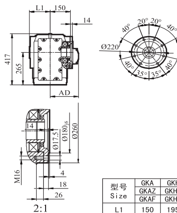
GKAF/GKHF/GKV97
