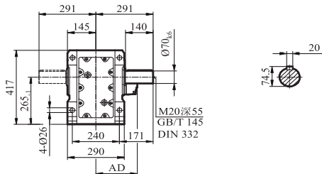
GKA/GKH/GKV97
