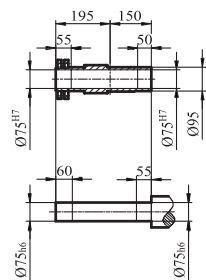
GKH/GKHZ/GKHF97输出轴
