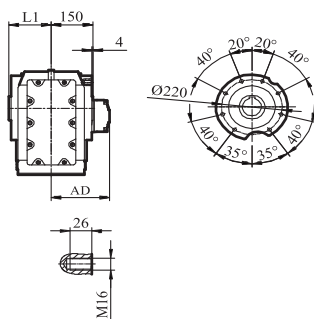
GKA/GKH/GKV97
