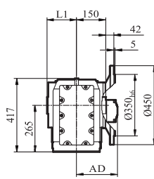
GKAF/GKHF/GKV97
